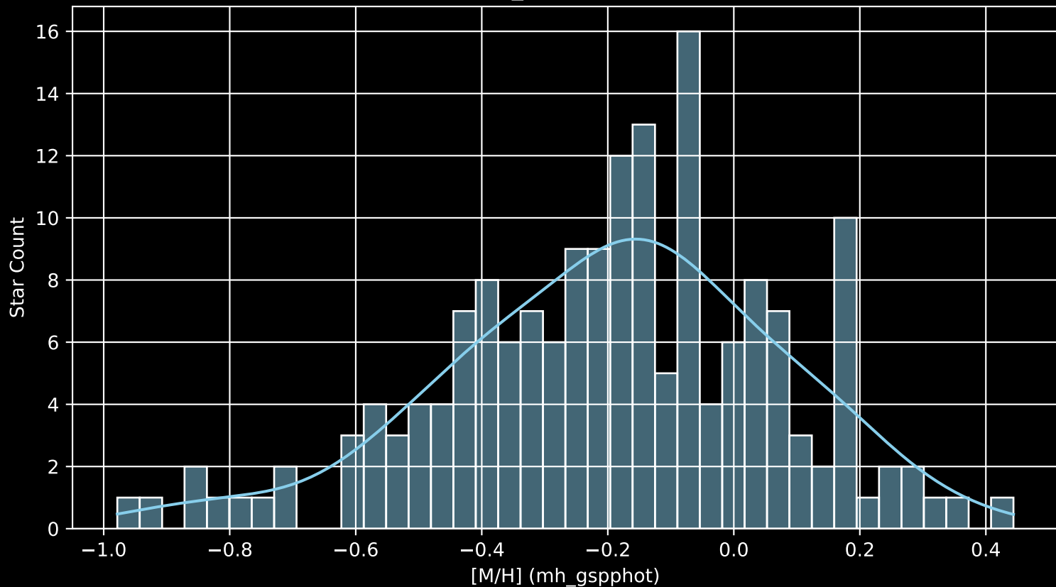
APOGEE DR17 Field: [068+55_MGA [M/H] (mh_gspphot) (n= 173)
