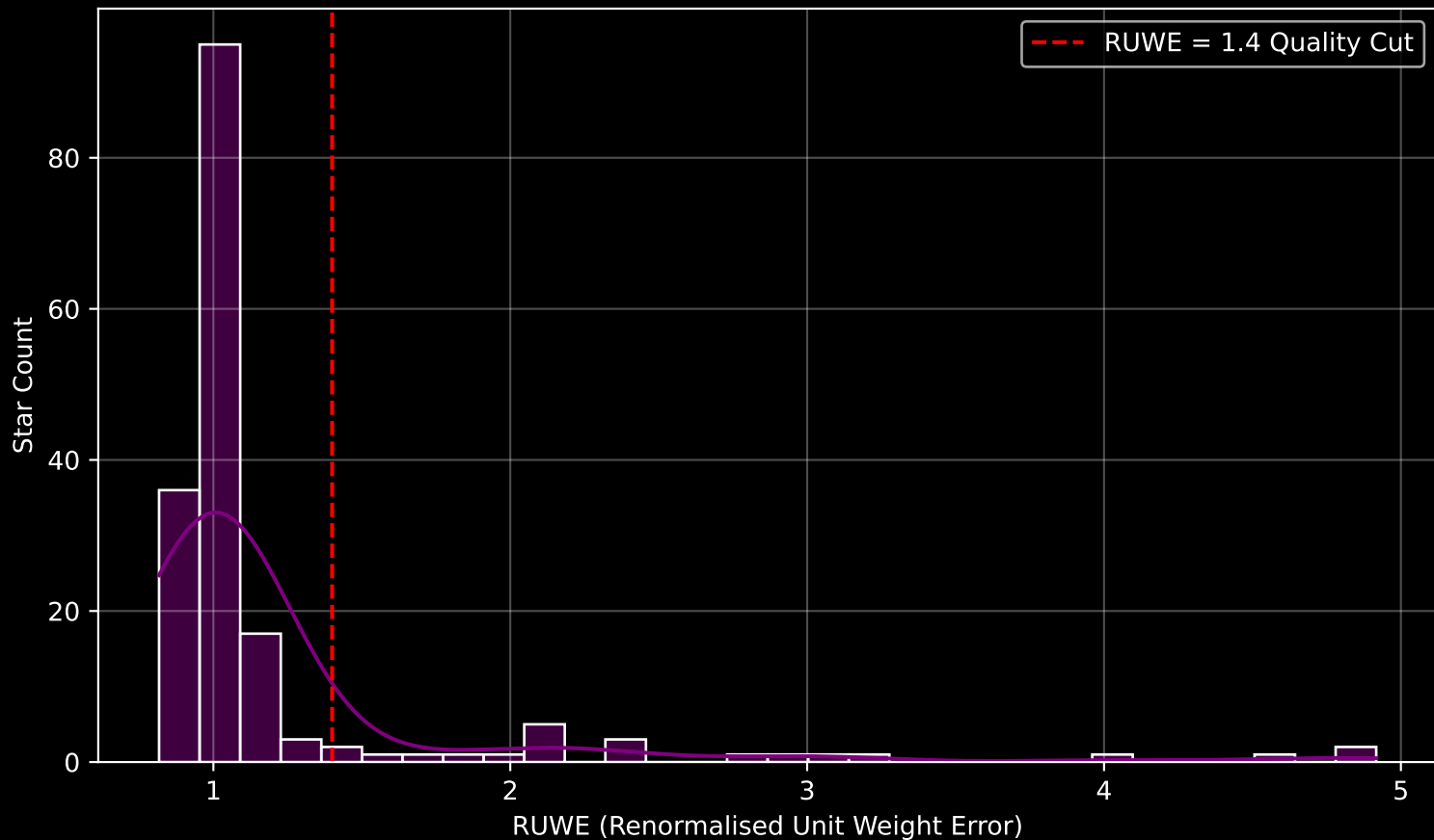
GAPOGEE DR17 Field [068+55_MGA] RUWE Distribution (n= 173)
