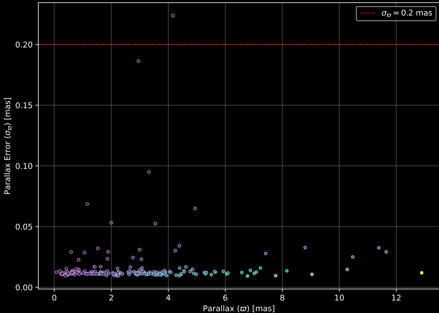
APOGEE DR17 Field: [068+55_MGA] Parallax Quality (n= 176)
