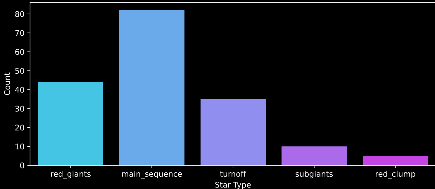
APOGEE DR17 Field: [068+55_MGA] Count plot of Star Type
