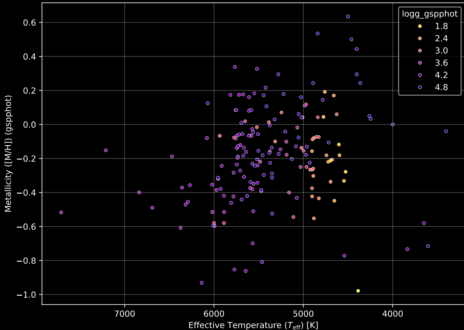
APOGEE DR17 Field: [068+55_MGA] Stellar Population Parameters (n= 176)
