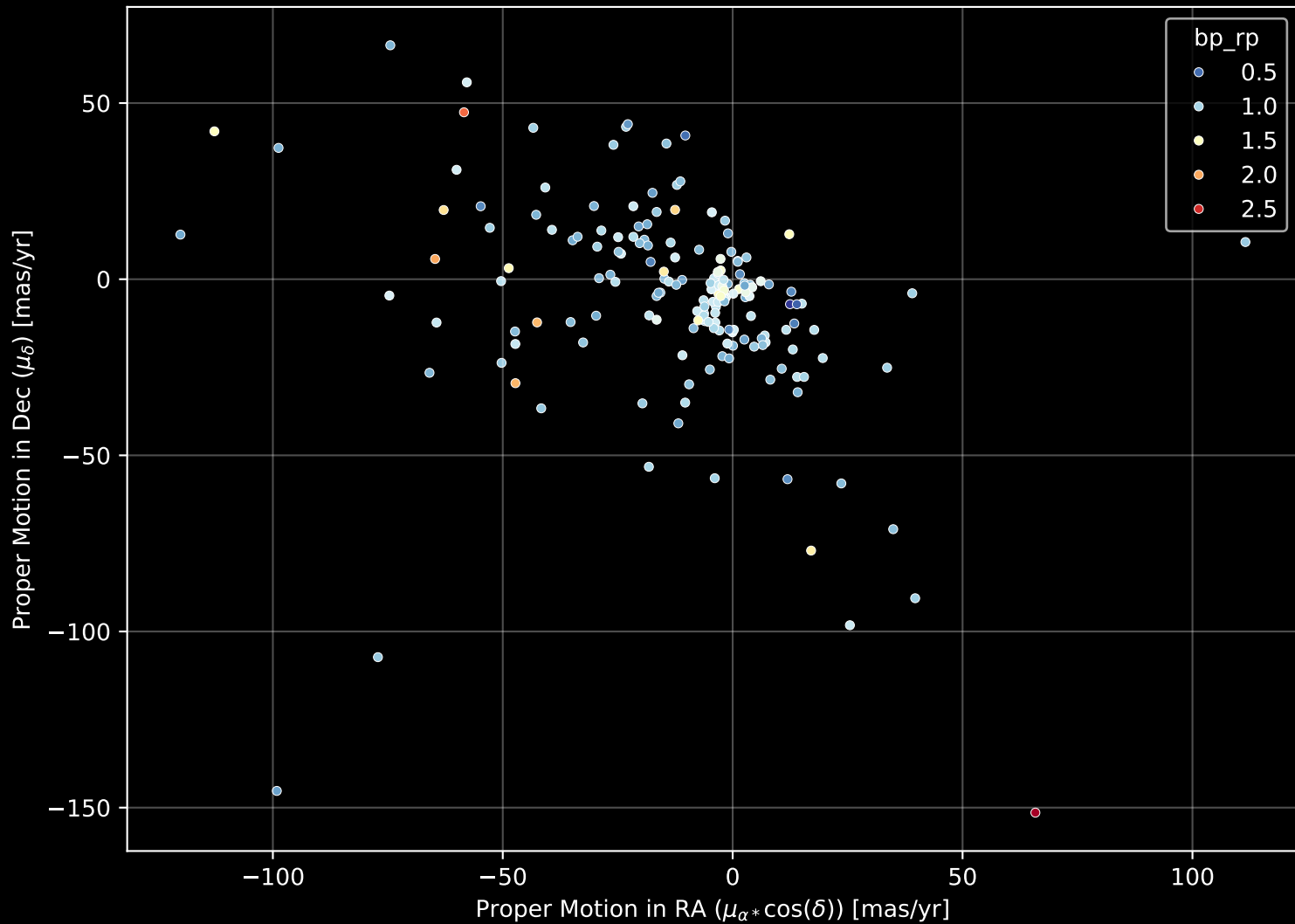
APOGEE DR17 Field: [068+55_MGA] Proper Motion Diagram (n= 176)
